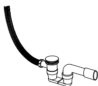
COLONNA SCARICO VASCA CON TROPPOPIENO INCLUSA / WASTE WITH OVERFLOW INCLUDED
